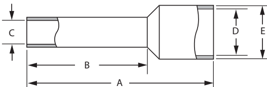
SINGLE WIRE
